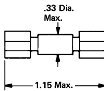
Model 70 3.5mm-M to 3.5mm-M
