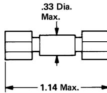
Model 60B SMA-M to SMA-M
